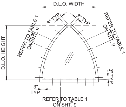
TYP. ANCHOR LAYOUT ON IRREGULAR SHAPE FRAME
